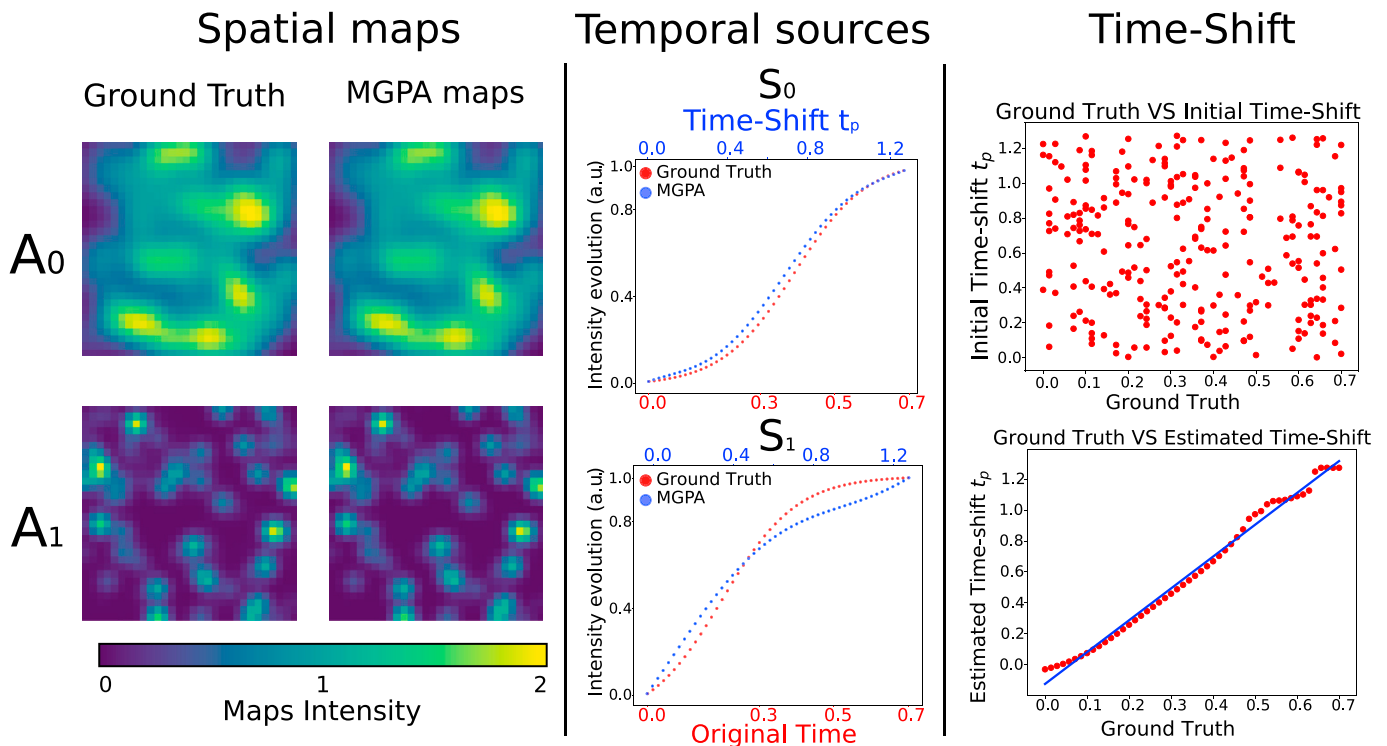
Fig. 5. Spatio-temporal reconstruction when inference on the time-line is required. Optimal reconstruction result. Spatial maps: Sample slice from ground truth images ( A_0 \lambda = 2 mm, A_1 \lambda = 1 mm) and estimated spatial sources. Temporal sources: In red the original temporal sources, in blue the estimated temporal sources. Time-Shift: Time-shift t_p of each image at initialization (top), and after estimation (bottom). In blue, linear fit with the ground truth.
